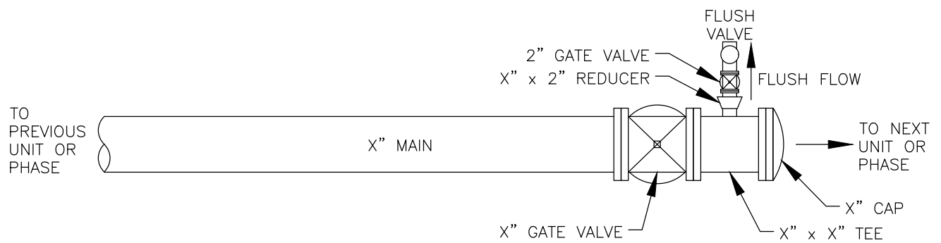
PLAN VIEW
